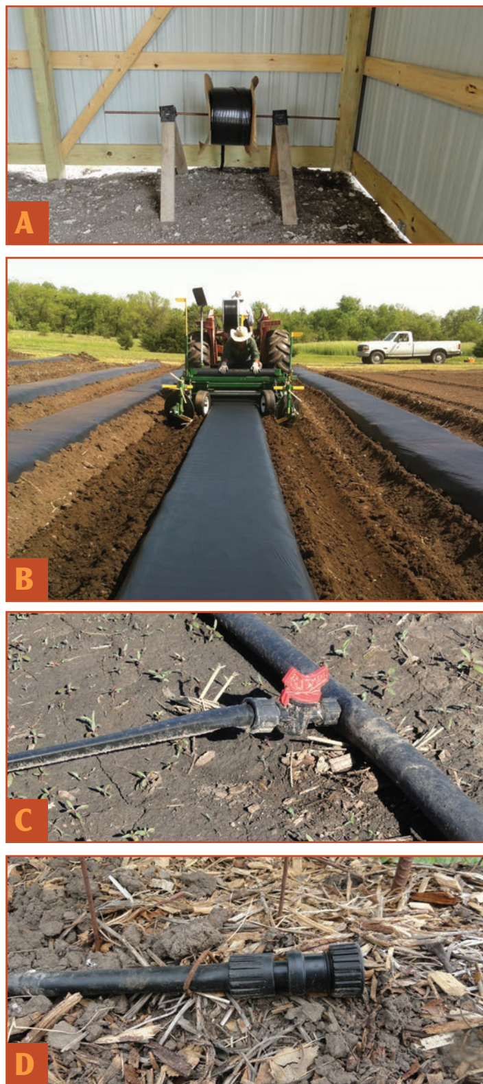
Figure 10. (A) A simple system for unrolling drip tape without kinks that can be used by a single installer. (B) A bed-shaper installs drip tape and plastic mulch. (C) Drip tape is connected to the header pipe with simple PVC connectors that have reverse-threaded locking collars (D). Drip tubing is terminated with a premanufactured cap.
