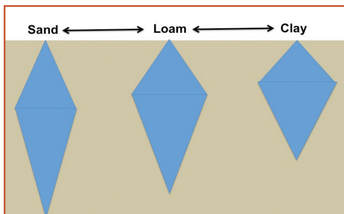
Figure 3. Distribution of water in various soil types. High concentrations of clay lead to wider distribution, and greater amounts of sand lead to narrow water distribution.
